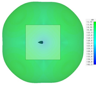
UHF-Element 380 MHz
