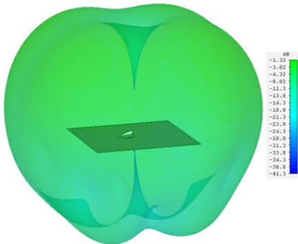
UHF-Element 380 MHz
