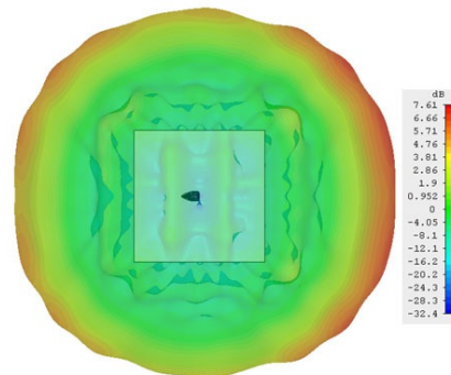
4G-Element 1800 MHz
