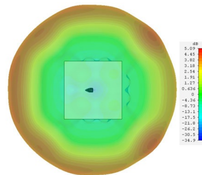
4G-Element 900 MHz
