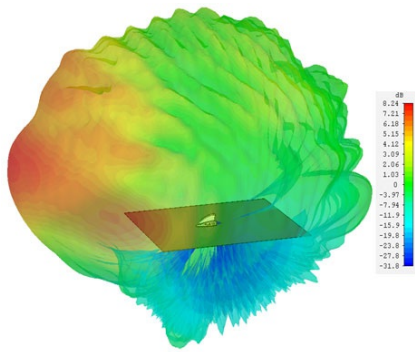
WIFI-Element 5600 MHz
