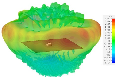
4G-Element 2600 MHz
