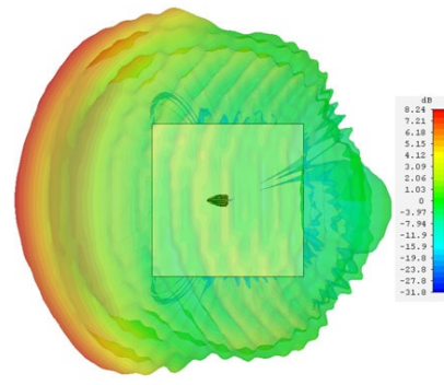
WIFI-Element 5600 MHz
