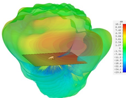
WIFI-Element 2400 MHz
