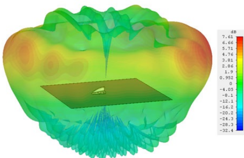
4G-Element 1800 MHz
